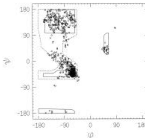
FIGURE 1: Ramachandran plot of dimeric yeast enolase main-chain non-glycyl dihedrals. Fully allowed \phi and \psi values are shown by solid enclosures. Partially allowed regions are enclosed by broken lines. Dihedral angles for the most severe outliers are distorted by hydrogen-bonding and ionic interactions. The most severe left-handed helical outlier in both subunits is Arg 402, whose guanidinium group interacts with Glu 404. The most severe right-handed outlier in both subunits is Asp 320, which interacts with \text{Mg}^{2+} .
